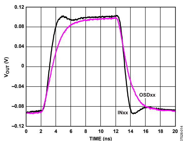
Figure 14. ADV3203 Small Signal Pulse Response, 200 mV p-p
