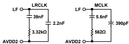
Figure 32. Recommended Loop Filters for LRCLK or MCLK as PLL Reference
