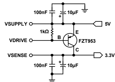
Figure 34. Recommended 3.3 V Regulator Circuit
