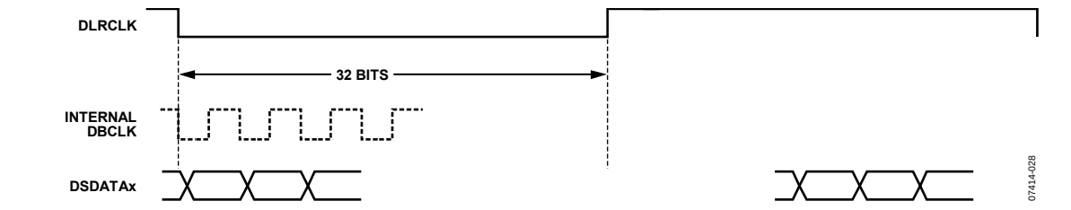
Figure 28. Serial DAC Data Transmission in TDM Format Without DBCLK; 2-Channel 64 BCLKs per Frame Mode (Applicable Only If PLL Locks to DLRCLK; This Mode Is Also Available in the ADC Serial Data Port)
