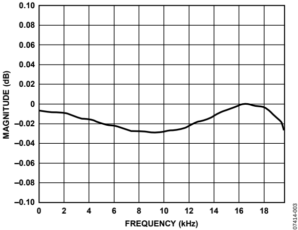
Figure 5. ADC Pass-Band Filter Response, 48 kHz
