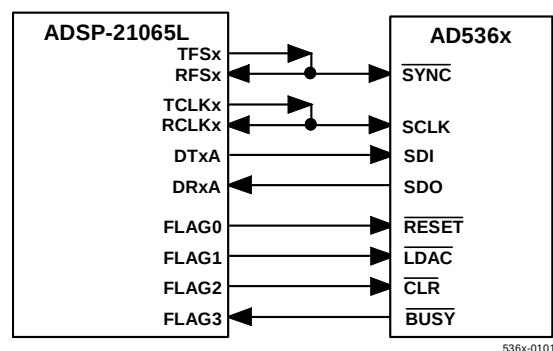
Figure 12. Interfacing to a ADSP-21065L DSP
