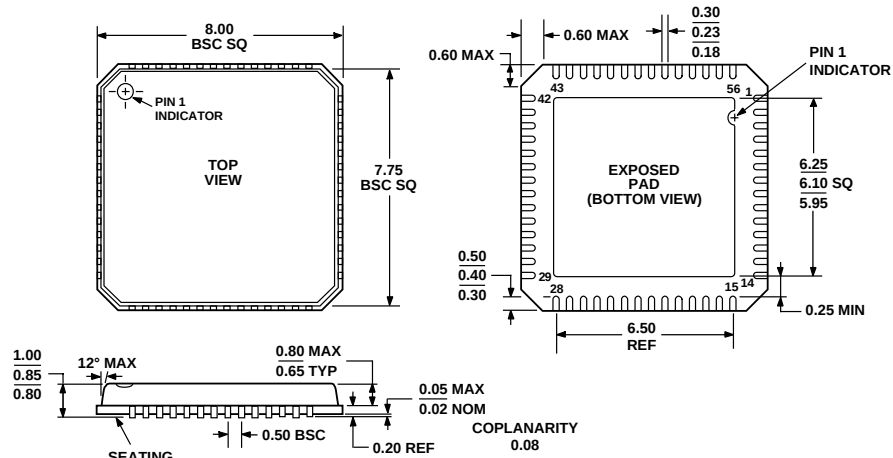
Figure 11. 56 Lead LFCSP Package Dimensions shown in millimeters
