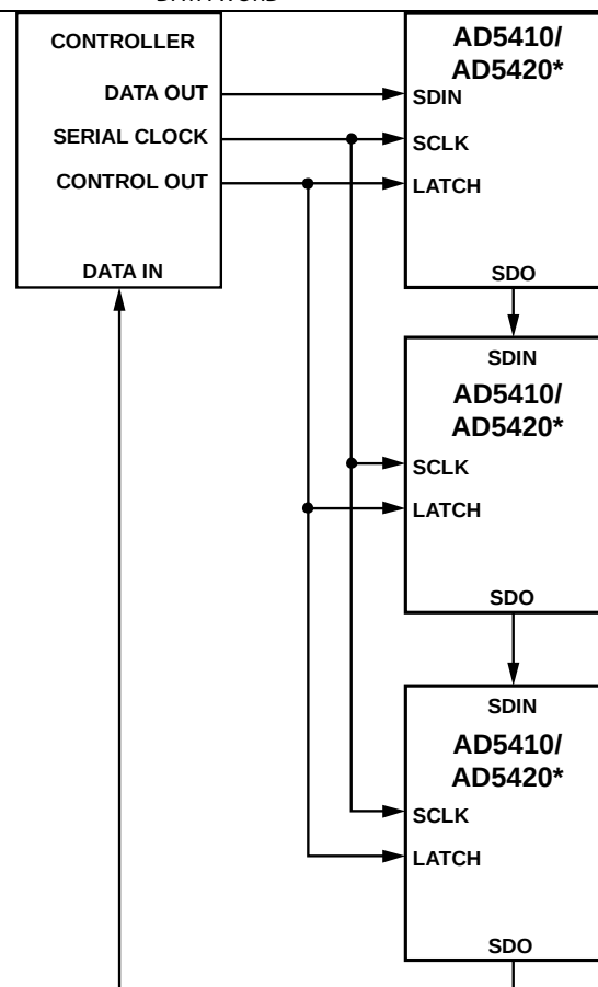
Figure 35. Daisy Chaining the AD5410/AD5420
