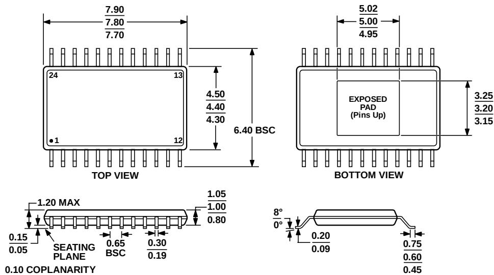
Figure 43. 24-Lead Thin Shrink Small Outline Package, Exposed Pad [TSSOP_EP] (RE-24)
