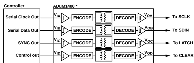
Figure 40. Isolated Interface
