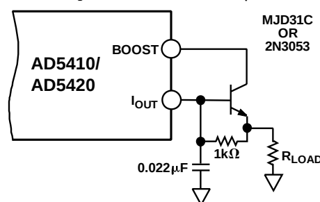
Figure 36. External Boost Configuration
