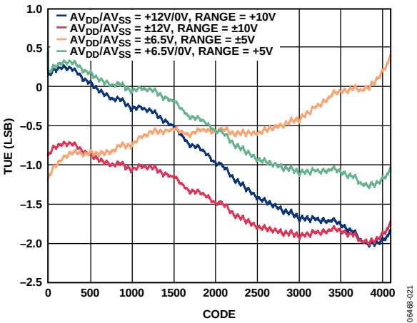
Figure 37. AD5724 Total Unadjusted Error vs. Code
