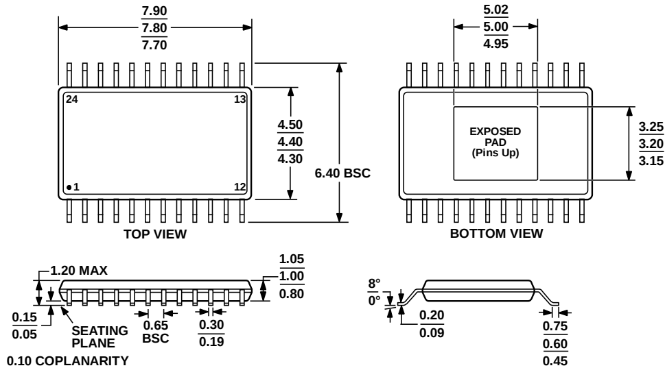
Figure 45. 24-Lead Thin Shrink Small Outline Package, Exposed Pad [TSSOP_EP] (RE-24) Dimensions shown in millimeters
