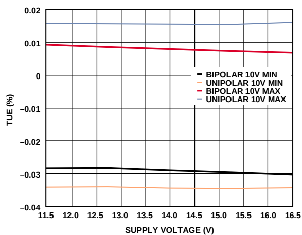
Figure 18. AD5754 Total Unadjusted Error vs. Supply Voltage
