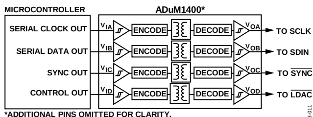
Figure 43. Isolated Interface
