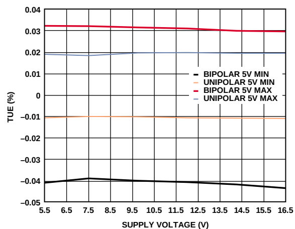
Figure 19. AD5754 Total Unadjusted Error vs. Supply Voltage
