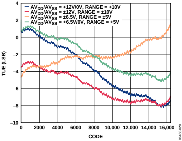
Figure 36. AD5734 Total Unadjusted Error vs. Code
