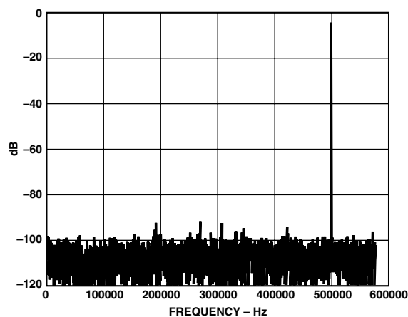
TPC 4. Typical SNR @ 500 kHz Input Tone
