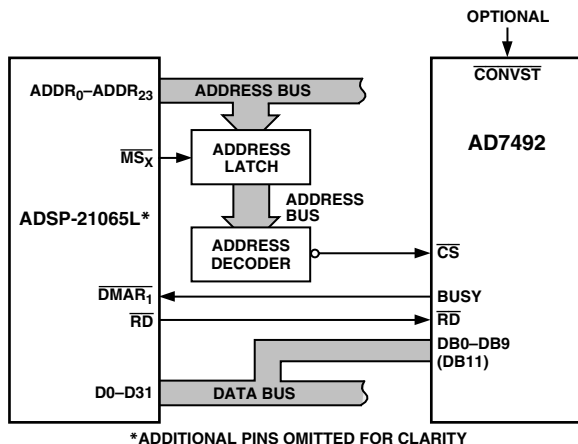
Figure 20. Interfacing to ADSP-21065L
