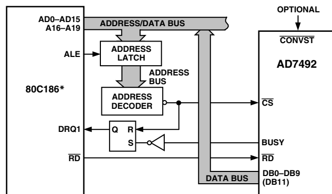
Figure 23. Interfacing to 80C186
