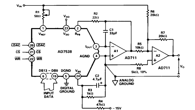
Figure 5. Bipolar Operation
