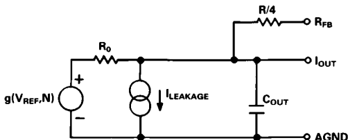
Figure 3. AD7538 Equivalent Analog Output Circuit
