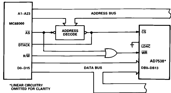
Figure 10. AD7538-MC68000 Interface
