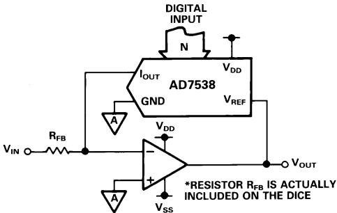
Figure 7. Programmable Gain Amplifier (PGA)
