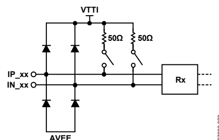
Figure 19. High Speed Input Simplified Schematic
