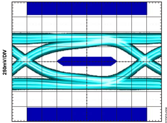
Figure 6. Rx Eye Diagram at TP2 (Cable = 6 m, 24 AWG)
