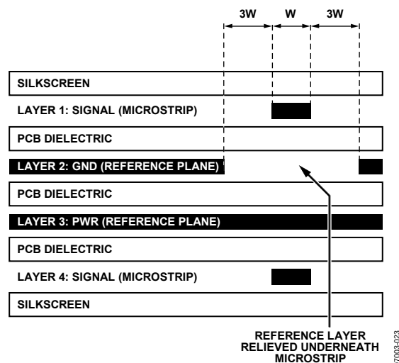
Figure 22. Example Board Stackup
