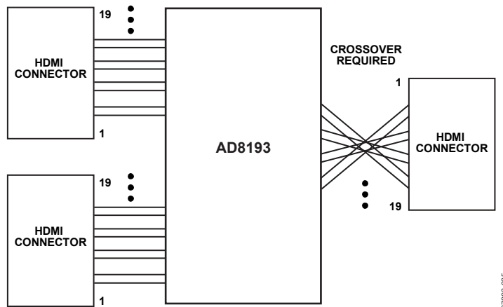
Figure 24. Block Diagram of AD8193 Evaluation Board Showing Output Crossover
