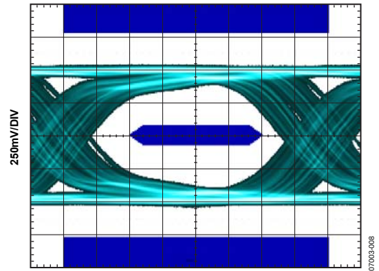
Figure 8. Rx Eye Diagram at TP3 (Cable = 6 m, 24 AWG)
