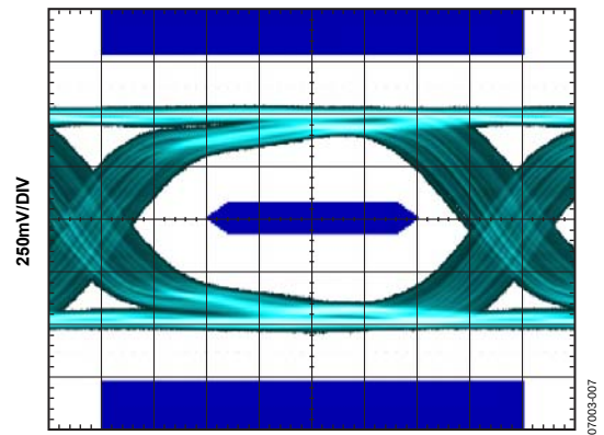
Figure 7. Rx Eye Diagram at TP3 (Cable = 2 m, 30 AWG)
