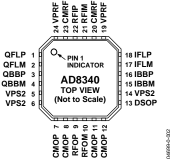
Figure 2. 24-Lead Lead Frame Chip Scale Package (LFCSP)
