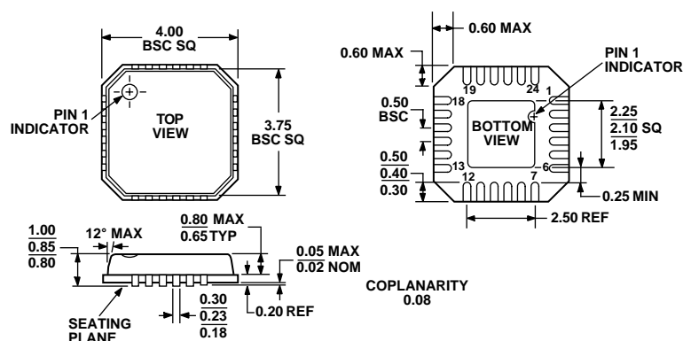
Figure 42. 24-Lead Lead Frame Chip Scale Package (LFCSP) (CP-24)
