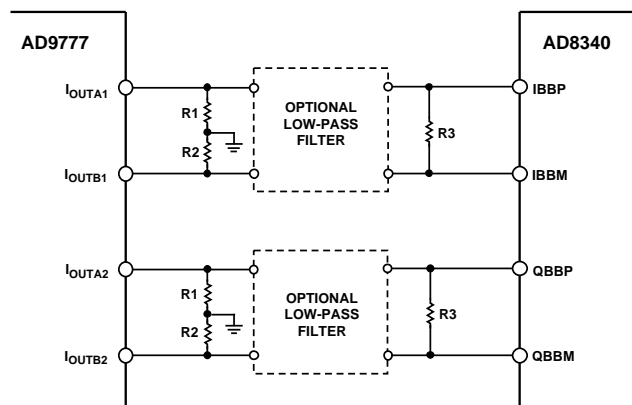
Figure 33. Basic AD9777 to AD8340 Interface
