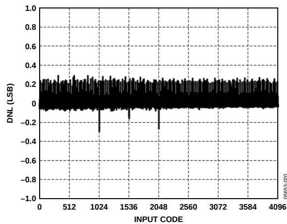
Figure 10. DNL vs. Code @ T_A = 25^\circ\text{C} , INV = L
