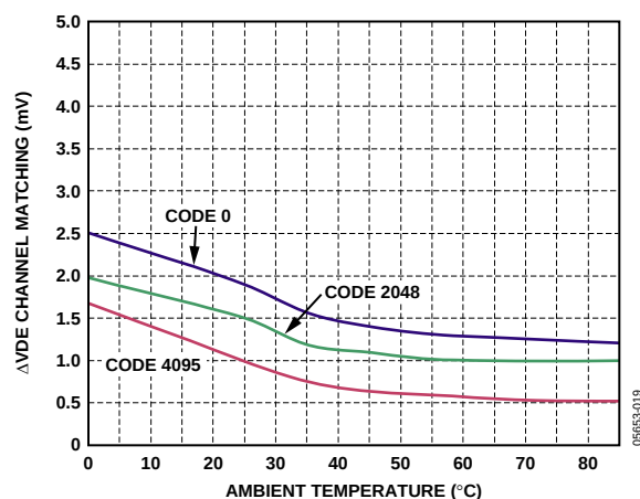
Figure 8. Channel Matching vs. T_A @ Codes 0, 2048, 4095
