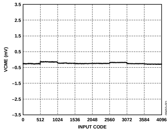
Figure 9. VCME vs. Code
