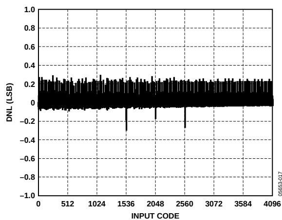
Figure 7. DNL vs. Code @ T_A = 25^\circ\text{C} , INV = H
