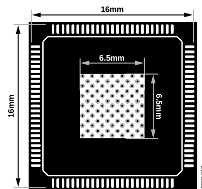
Figure 18. Land Pattern—Top Layer
