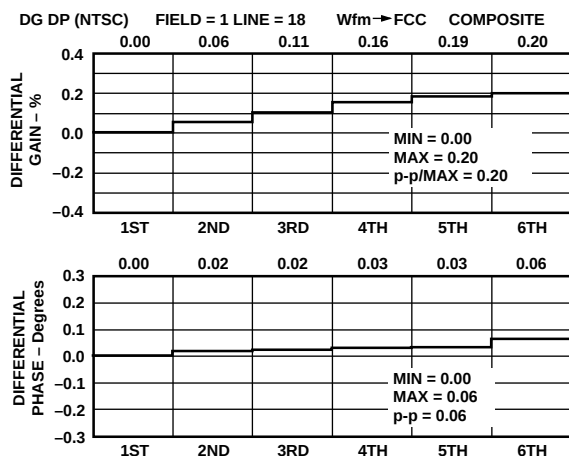
Figure 1. Typical Composite Output Differential Gain & Phase, NTSC for X Channel; f = 3.58 MHz, R_L = 150\ \Omega
