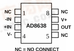
8- Lead SOIC (R-8 Suffix)
