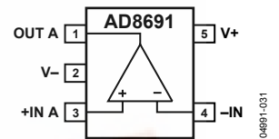
Figure 2. 5-Lead SC70
