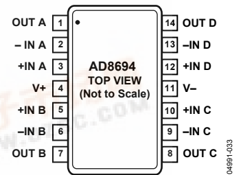
Figure 6. 14-Lead TSSOP
