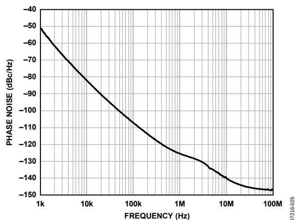
Figure 25. Internal VCO Phase Noise (Absolute), Direct-to-LVPECL @ 2250 MHz
