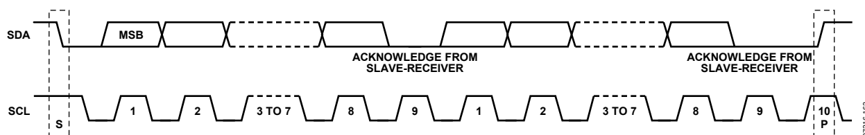
Figure 57. Acknowledge Bit
