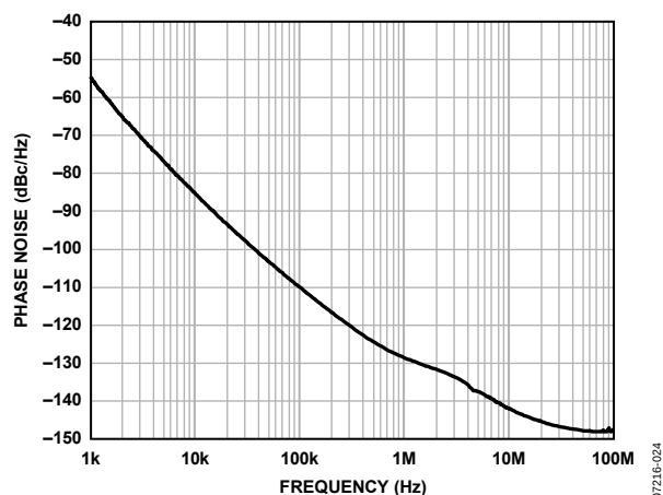
Figure 24. Internal VCO Phase Noise (Absolute), Direct-to-LVPECL @ 2000 MHz
