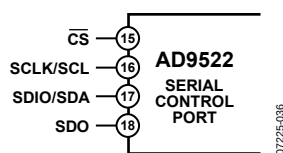
Figure 62. Serial Control Port
