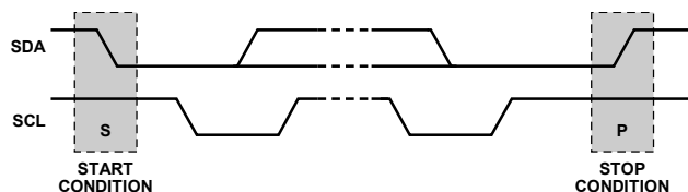
Figure 57. Start and Stop Conditions
