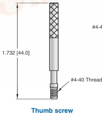
Thumb screw
