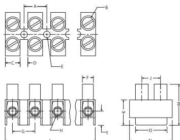
Dimensions mm
