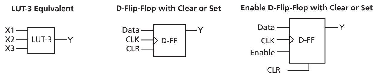
Figure 1-3 • VersaTile Configurations
