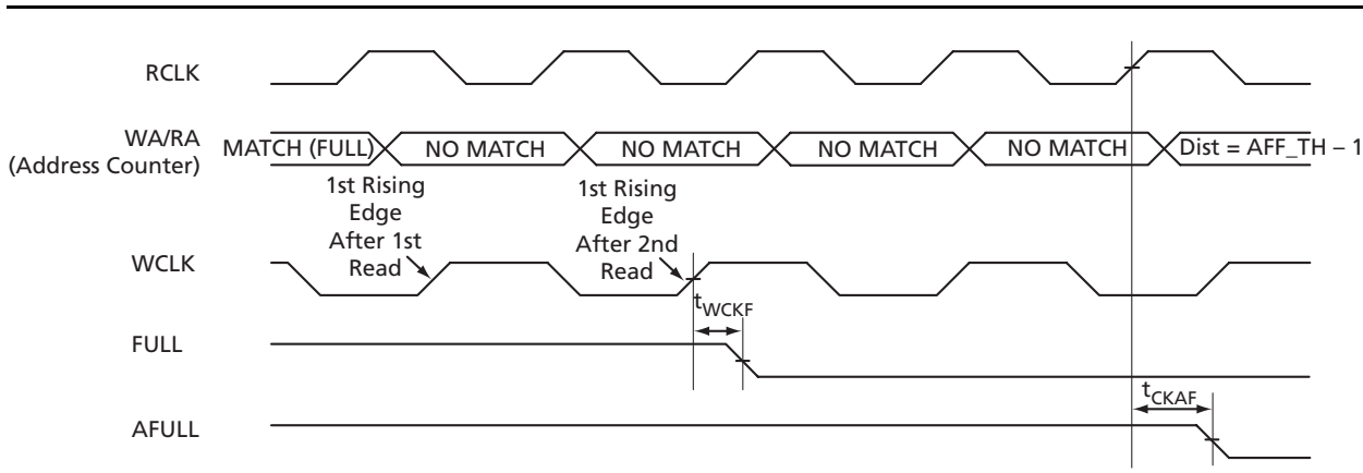
Figure 2-55 • FIFO FULL Flag and AFULL Flag Deassertion
