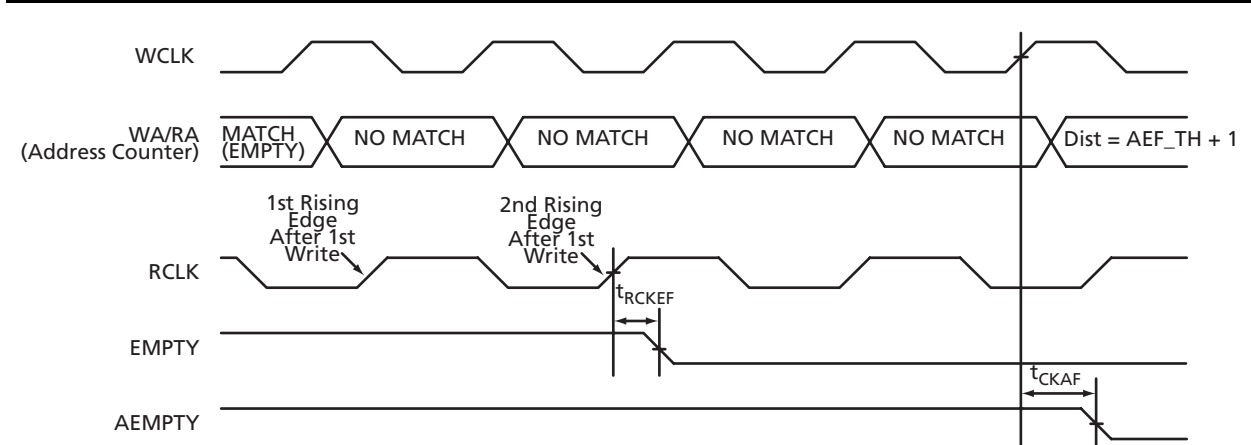
Figure 2-54 • FIFO EMPTY Flag and AEMPTY Flag Deassertion
