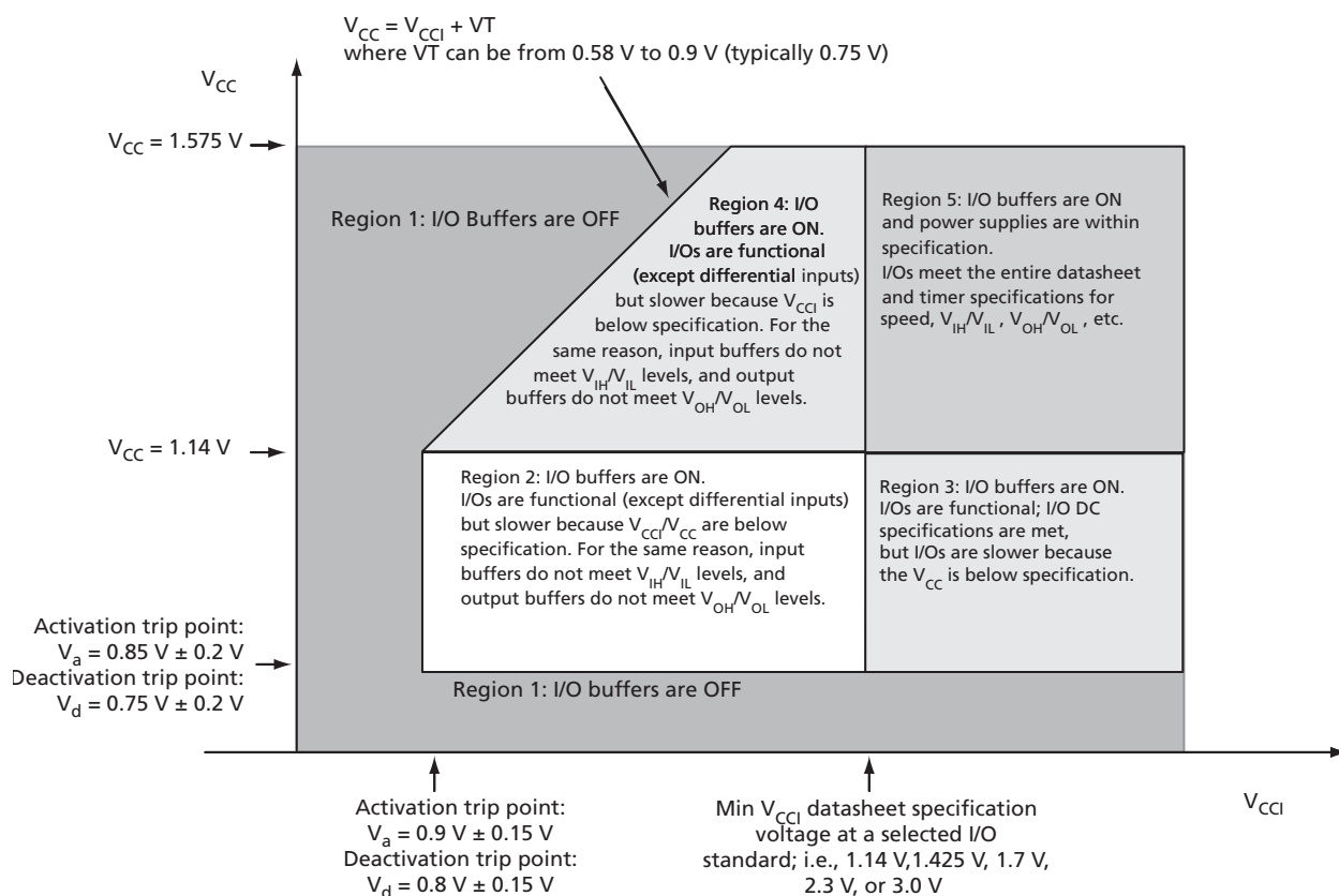
Figure 2-2 • V2 Devices – I/O State as a Function of V_{CC1} and V_{CC} Voltage Levels
