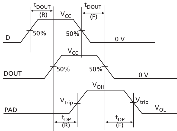
Figure 2-5 • Output Buffer Model and Delays (example)
