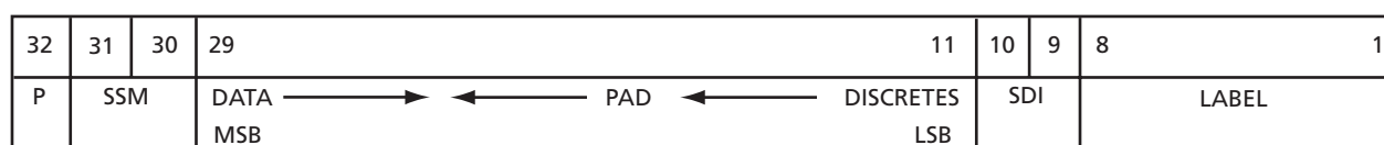
Figure 3 • ARINC Data Bit Positions
