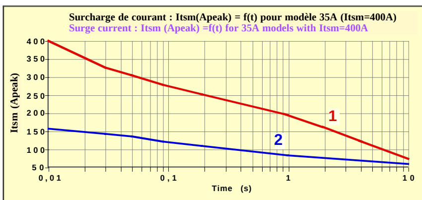
fig 3 : Courants de surcharges / Overload currents
