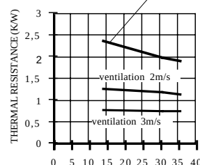
THERMAL RESISTANCE AIR CALM
