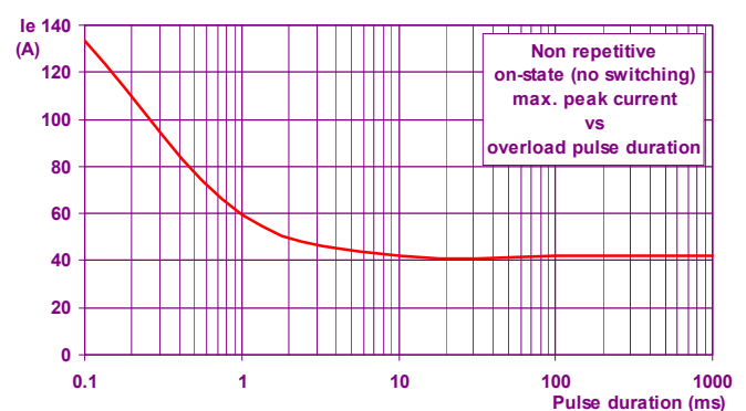
Fig. 8 CURRENT OVERLOAD CHARACTERISTIC
