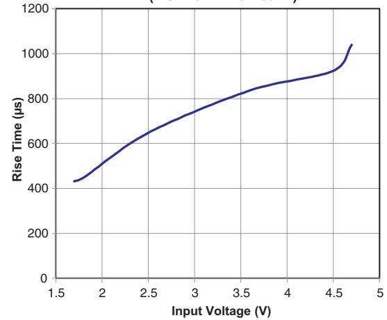
Rise Time vs. Input Voltage (AOZ1321DI-01L/04L)
