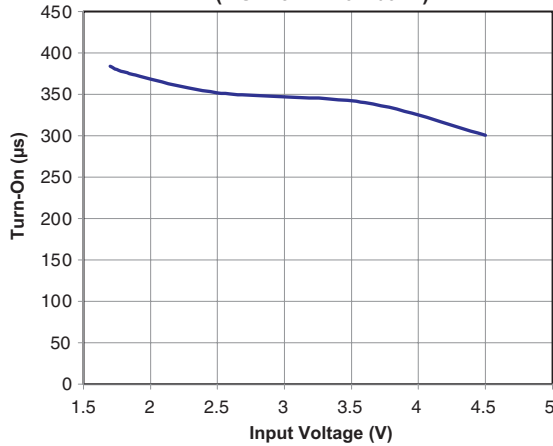
Turn-on Delay vs. Input Voltage (AOZ1321DI-01L/04L)
