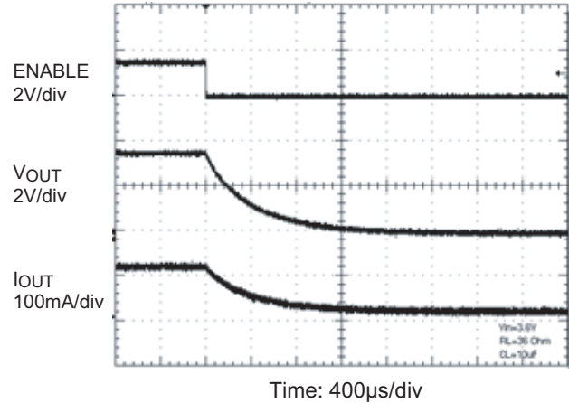
Turn-Off Timing
