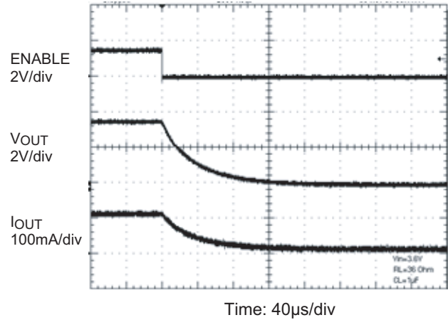
Turn-Off Timing
