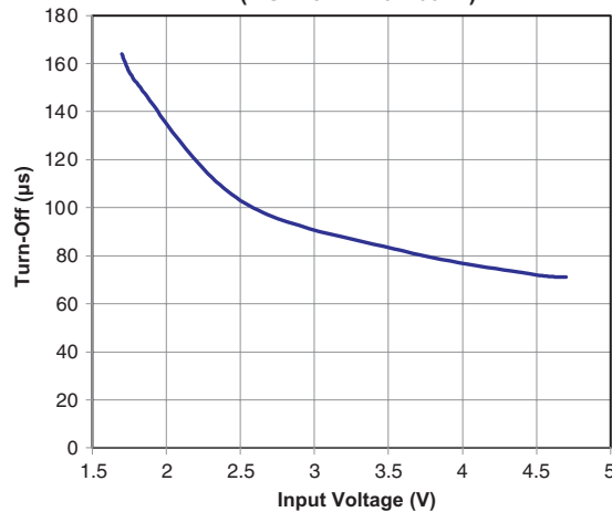
Turn-off Delay vs. Input Voltage (AOZ1321DI-01L/04L)
