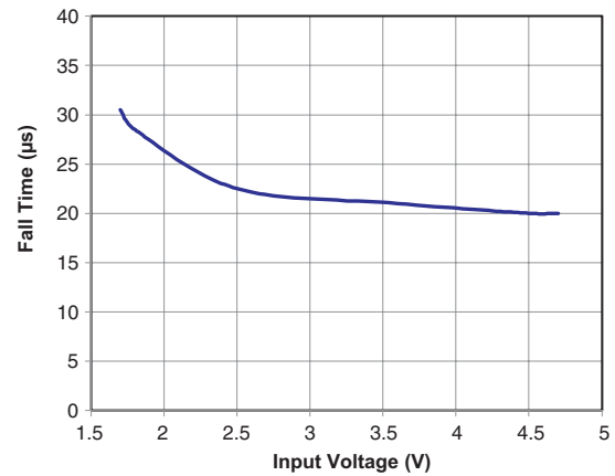
Fall Time vs. Input Voltage (AOZ1321DI-02L/05L)
