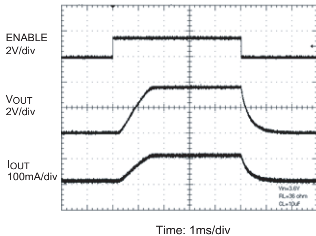
Turn-On/Turn-Off Timing
