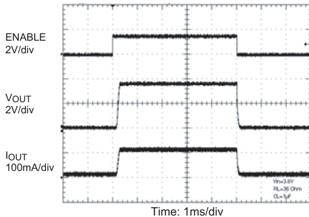
Turn-On/Turn-Off Timing
