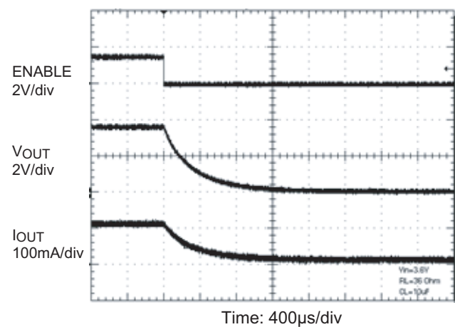
Turn-Off Timing
