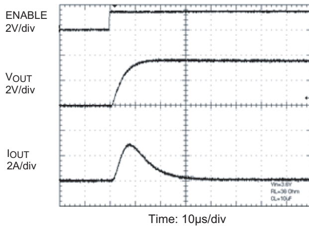
Turn-On Timing
