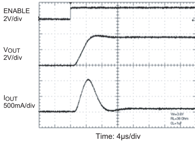
Turn-On Timing
