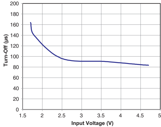
Turn-off Delay vs. Input Voltage (AOZ1321DI-02L/05L)
