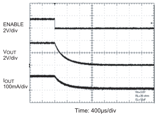
Turn-Off Timing
