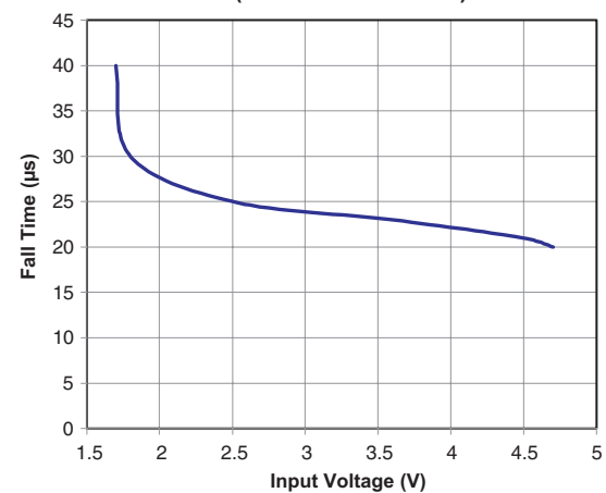
Fall Time vs. Input Voltage (AOZ1321DI-01L/04L)
