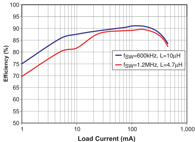
AOZ1905 Efficiency ( V_{IN} = 3.3V , V_{OUT} = 12V )
