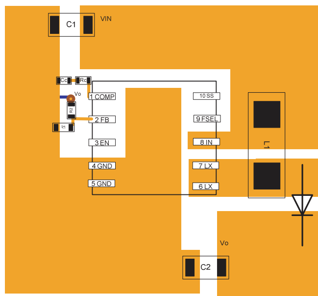
(a) DFN-10 3x3
