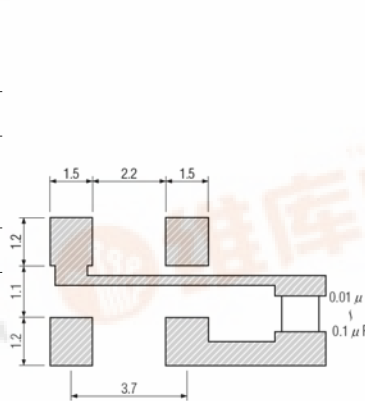
Figure 2) Suggested Land Pattern
