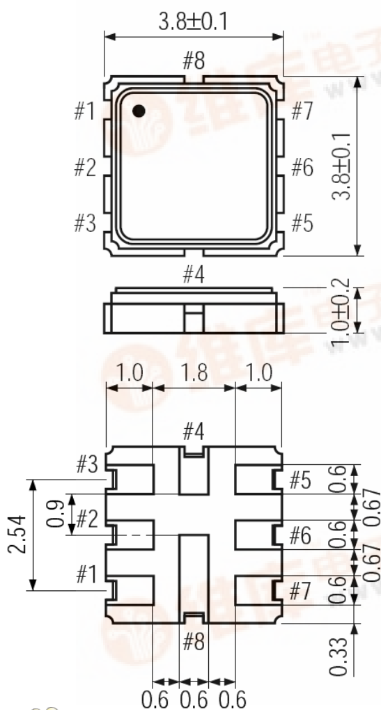
Figure 1) Top, Side and Bottom Views
