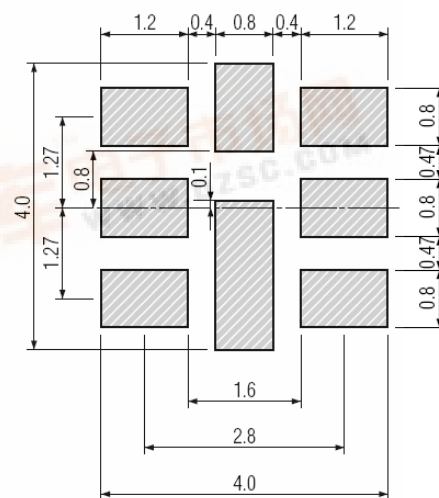
Figure 2) Land Pattern
