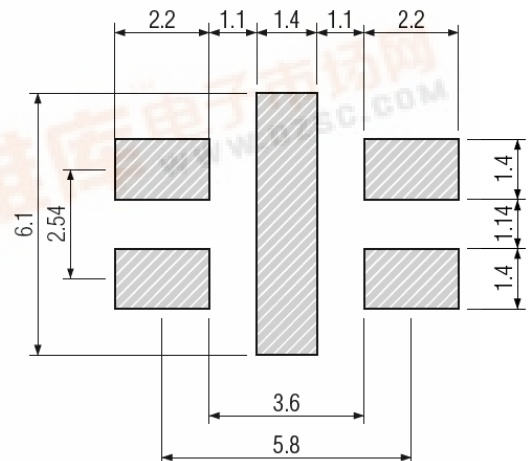
Figure 3) Land Pattern
