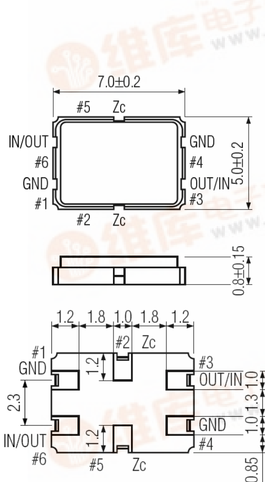
Figure 1) Top, Side and Bottom Views
