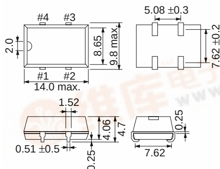
Figure 1) ECS-8F Top and Side view
