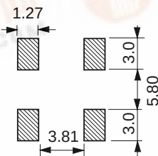
Figure 2) Land Pattern
