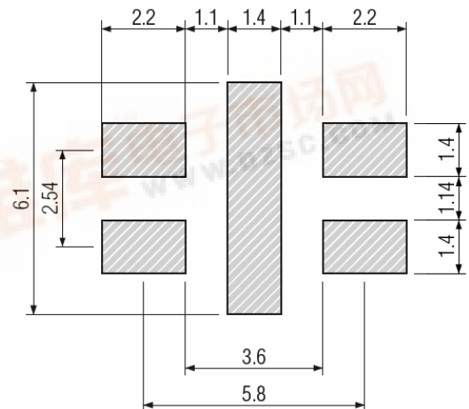
Figure 2) Land Pattern
