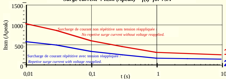
Fig.3: Surchage de courant : I_{tsm} (A_{peak}) = f(t) pour modèle 75A/ Surge current : I_{tsm} (A_{peak}) = f(t) for 75A
