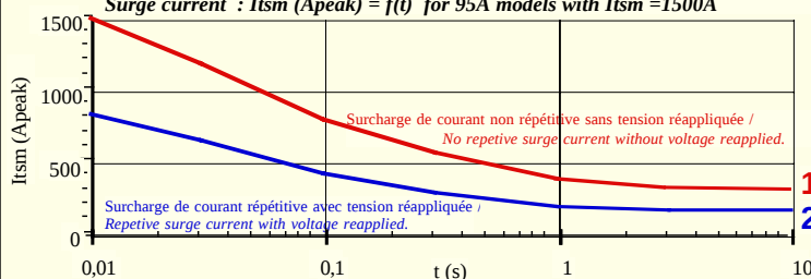
Fig.3 Surcharge de courant : I_{tsm} (A_{peak}) = f(t) pour modèle 95A ( I_{tsm}=1500A ) Surge current : I_{tsm} (A_{peak}) = f(t) for 95A models with I_{tsm}=1500A
