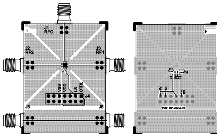
Figure 16. Evaluation Board Layouts
