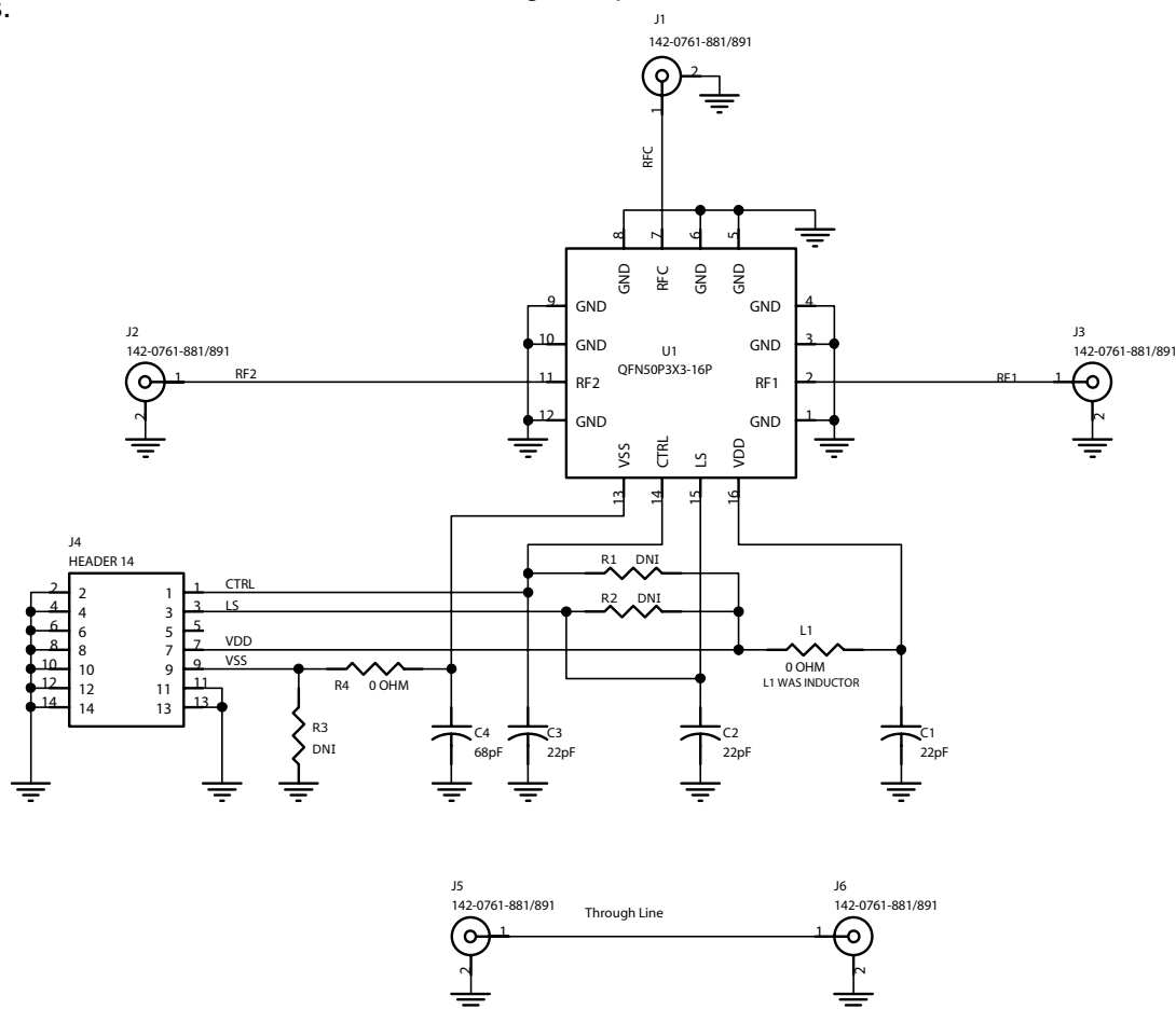
Figure 17. Evaluation Board Schematic
