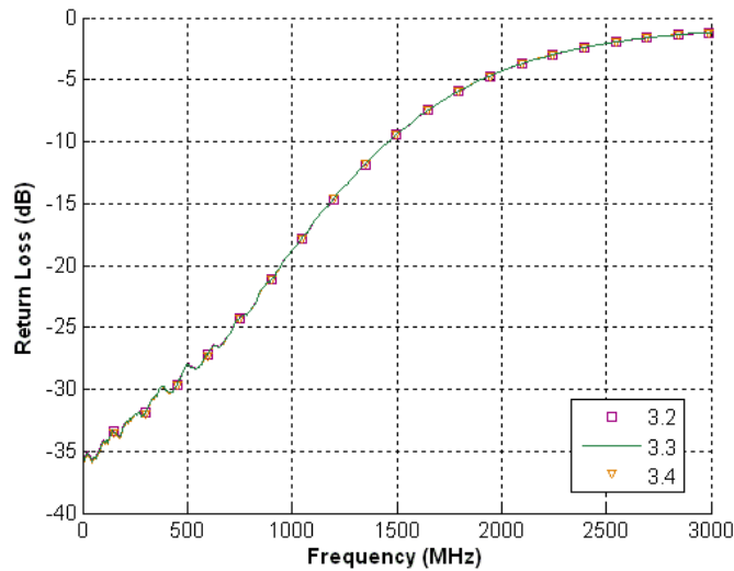
Figure 19. Tx Return Loss, +25°C
