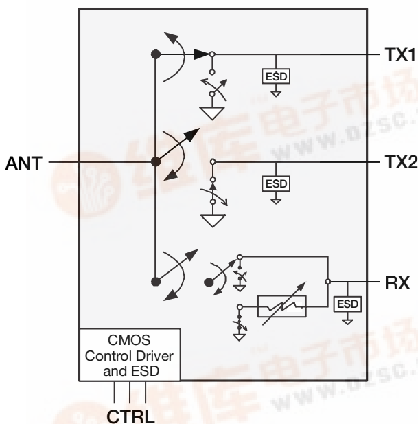
Figure 1. Functional Diagram
