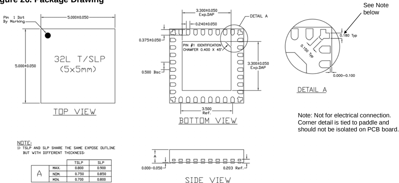
Figure 26. Package Drawing
