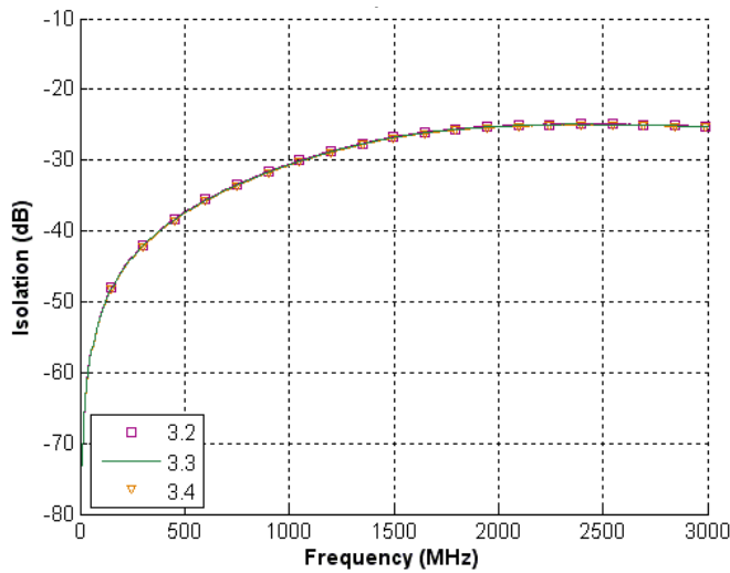
Figure 8. Isolation, Tx-Tx, +25°C
