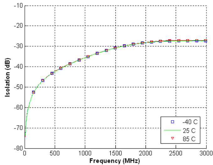
Figure 7. Isolation, Tx-Rx, V_{DD}=3.3V
