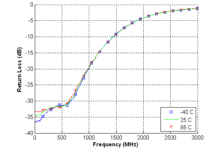
Figure 16. Return Loss, V_{DD}=3.3V
