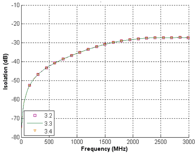
Figure 9. Isolation, Tx-Rx, +25°C
