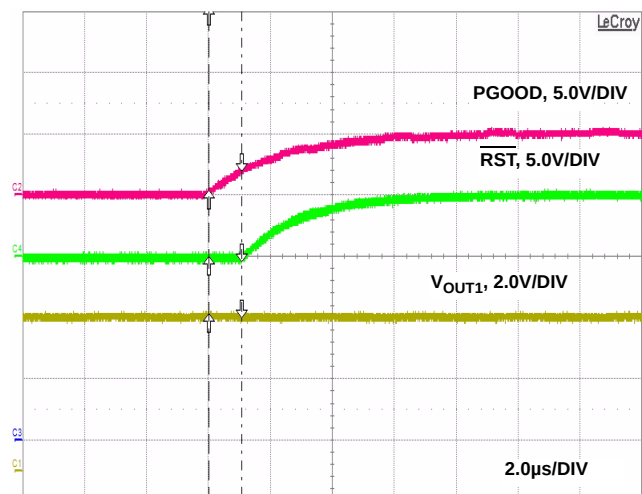
FIGURE 18. PGOOD RISING TO RST RISING
