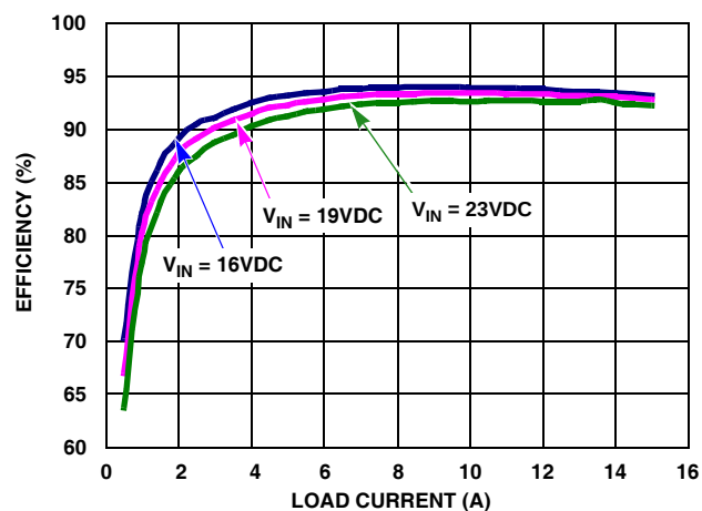
FIGURE 5. PWM2 EFFICIENCY vs LOAD ( V_O = 3.3V ), RJK0305DPB FOR UPPER MOSFET AND RJK0301DPB FOR LOWER MOSFET
