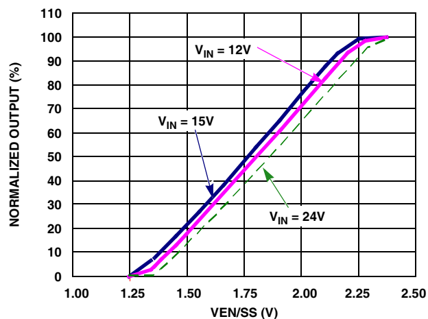
FIGURE 11. NORMALIZED OUTPUT VOLTAGE vs VEN/SS
