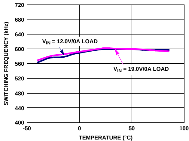
FIGURE 39. SWITCHING FREQUENCY vs TEMPERATURE
