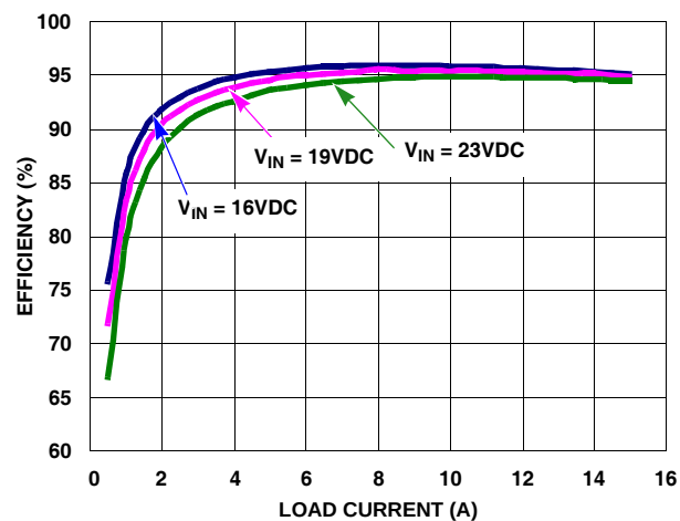
FIGURE 3. PWM1 EFFICIENCY vs LOAD ( V_{\text{O}} = 5.0\text{V} ), RJK0305DPB FOR UPPER MOSFET AND RJK0301DPB FOR LOWER MOSFET
