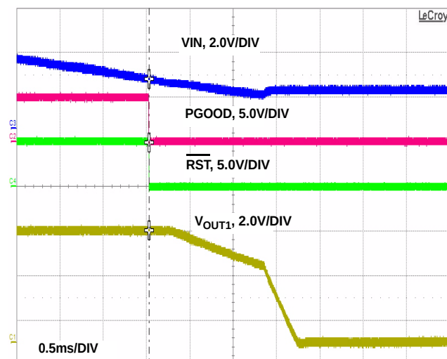
FIGURE 19. VIN FALLING TO PGOOD FALLING DELAY TIME
