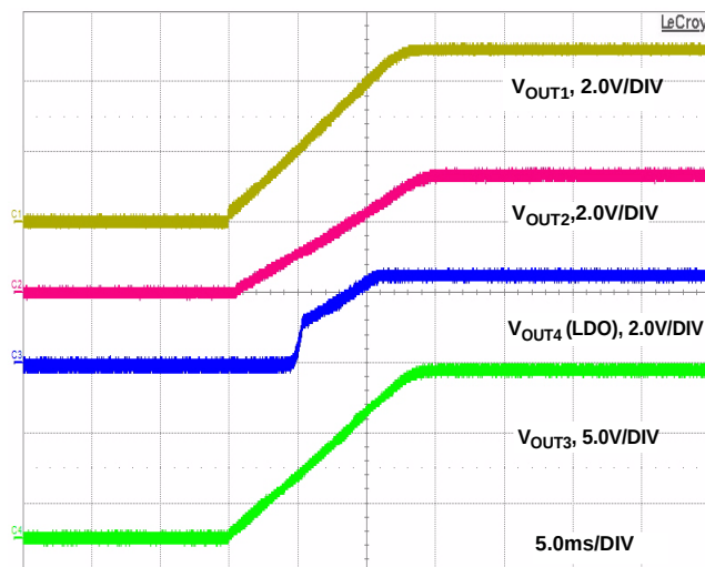
FIGURE 13. PWM SOFT-START WAVEFORMS, C_{SS} = 22nF
