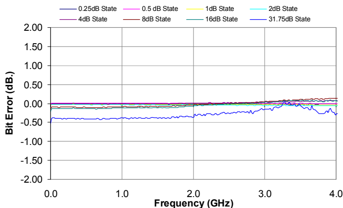
Figure 5. 0.25 dB Major State Bit Error
