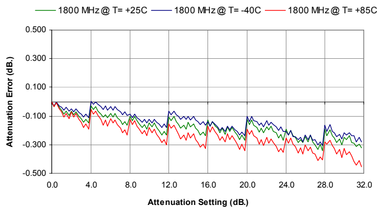
Figure 24. Attenuation Error vs. Attenuation Setting @ 1800 MHz
