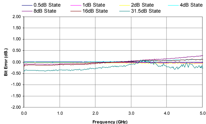
Figure 9. 0.5 dB Major State Bit Error
