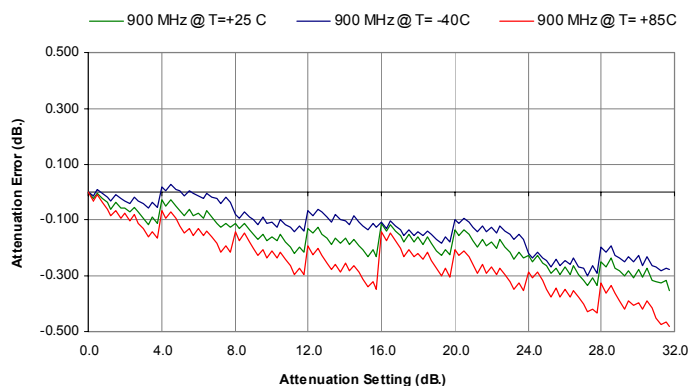
Figure 23. Attenuation Error vs. Attenuation Setting @ 900 MHz
