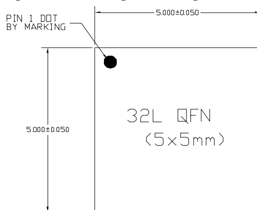
Figure 33. Package Drawing
