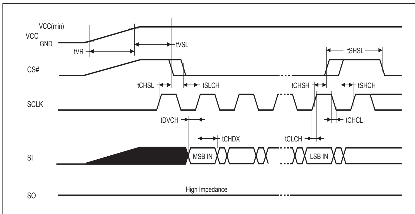
Figure A. AC Timing at Device Power-Up
