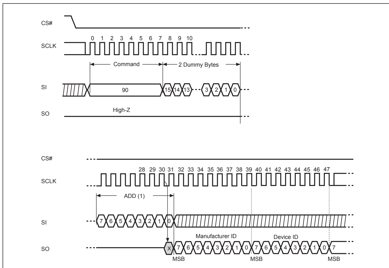
Figure 30. Read Electronic Manufacturer & Device ID (REMS) Sequence (Command 90 or EF or DF)
