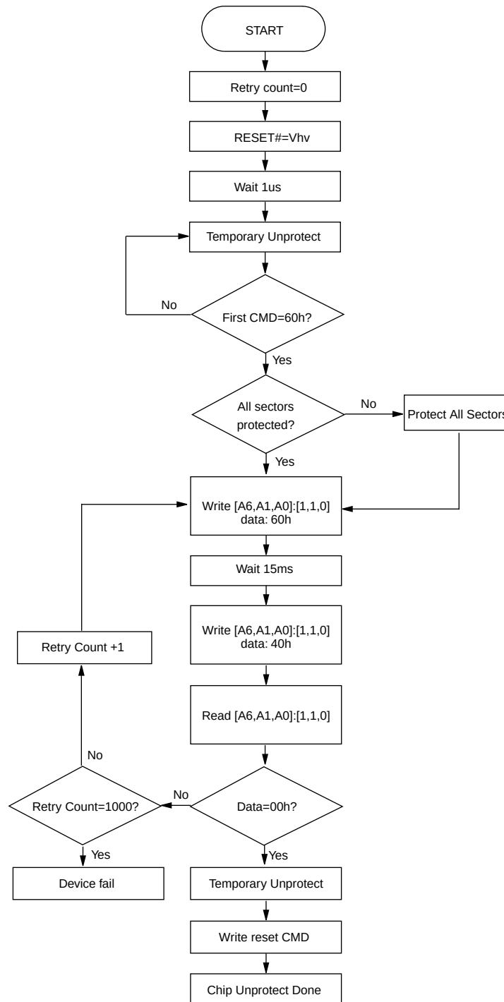
Figure 14-2. CHIP UNPROTECT ALGORITHMS WITH RESET# = V h v
