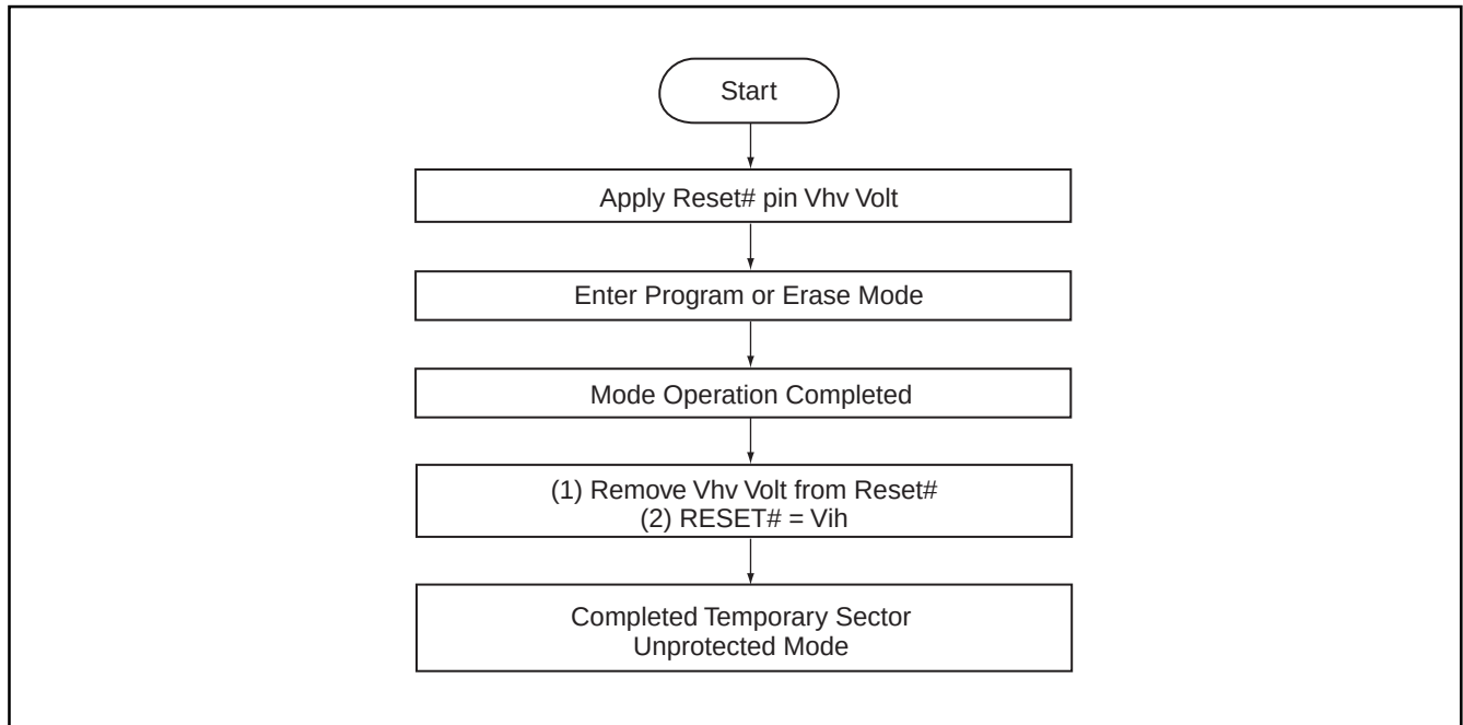
Figure 16. TEMPORARY SECTOR GROUP UNPROTECT FLOWCHART
