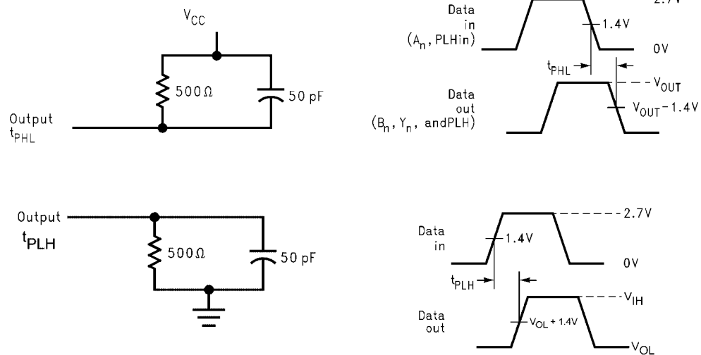
FIGURE 3. Port A to B and A to Y Propagation Delay Waveforms
