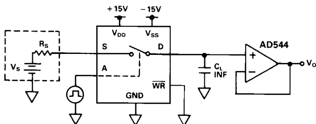
TEST CIRCUIT 7 CHARGE INJECTION
