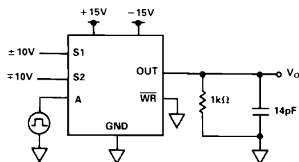
TEST CIRCUIT 6 SWITCHING TIME OF AD7592DI, t_{TRANSITION}
