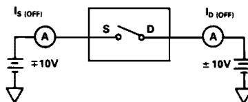
TEST CIRCUIT 2 (AD7590DI, AD7591DI)
