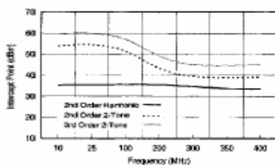
Intercept Point
