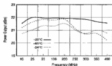
Power Output (1dB Gain Compression)
