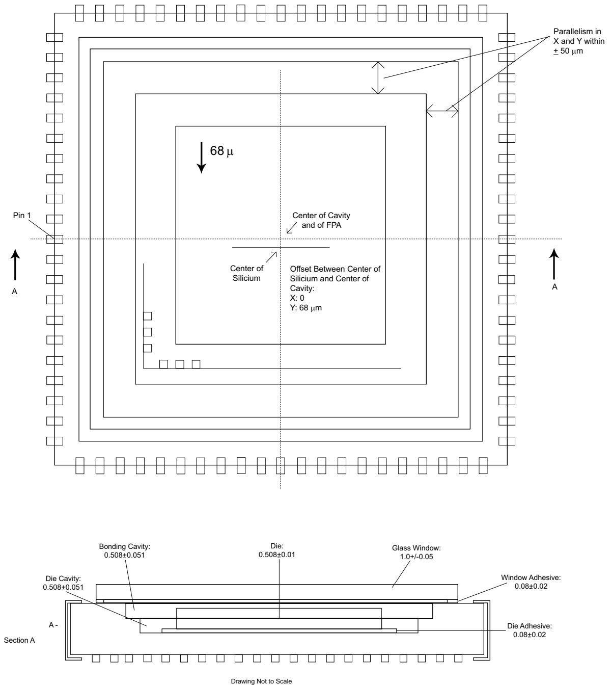
Figure 13. Die Alignment
