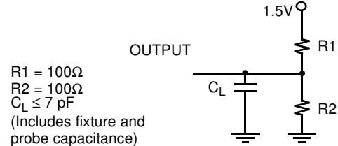
(c) HSTL AC Test Load
