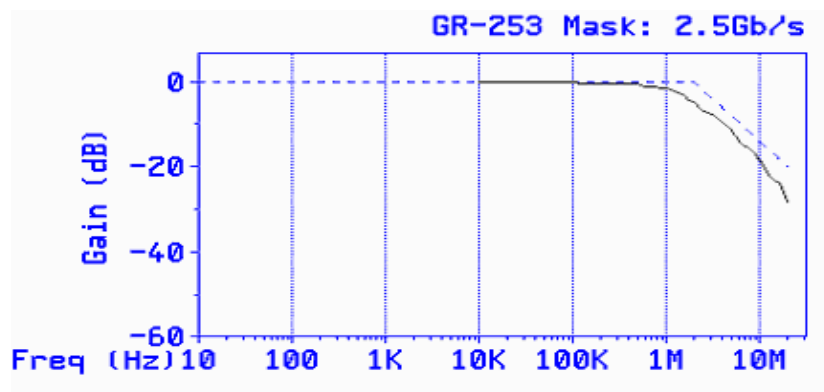
Figure 4. Jitter Transfer Waveform of CYS25G0101DX
