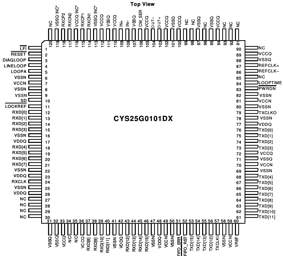
Figure 2. 120-Pin Thin Quad Flatpack Pin Configuration
