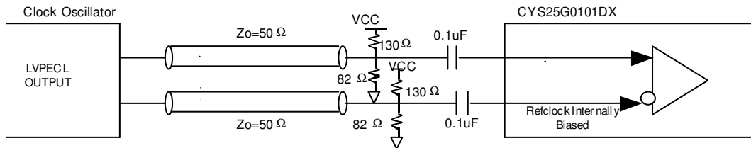
Figure 12. AC Coupled Clock Oscillator Termination
