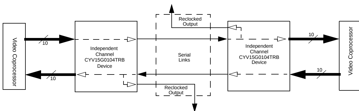
Figure 1. HOTLink II™ System Connections
