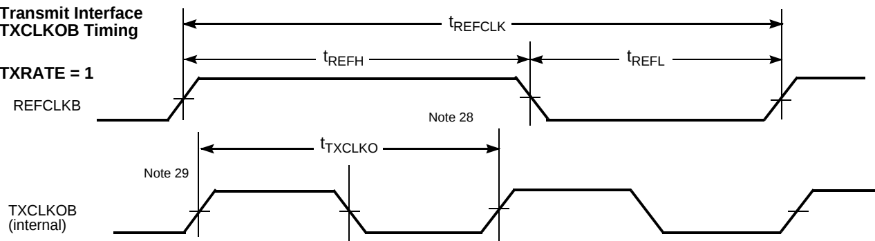
Transmit Interface TXCLKOB Timing
