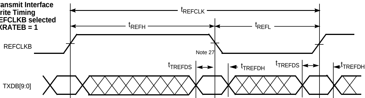
Transmit Interface TXCLKOB Timing
