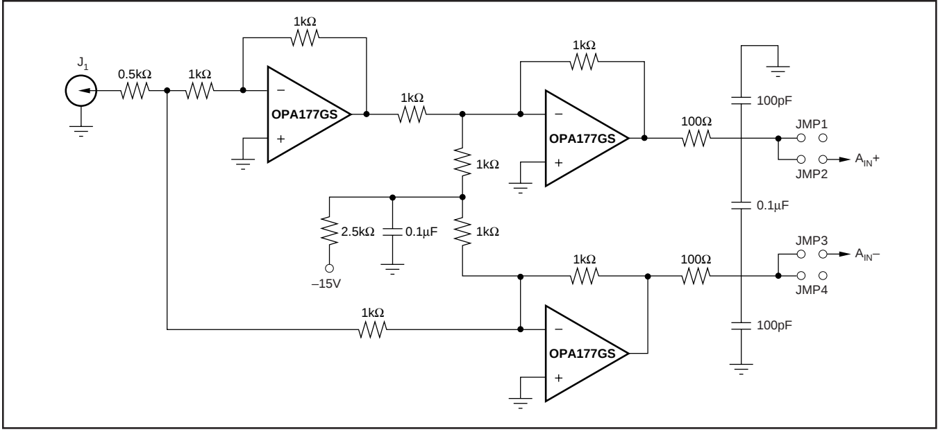
FIGURE 3. Analog Input Buffers.
