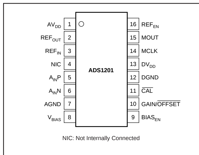
FIGURE 1. ADS1201U Device Pinout.
