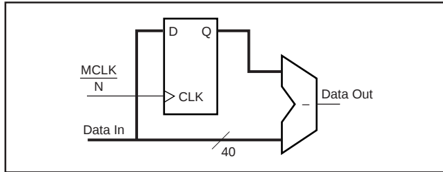
FIGURE 7. Xilinx Differentiator Implementation.
