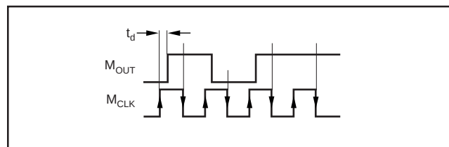
FIGURE 2. ADS1201U Output Read Operation.
