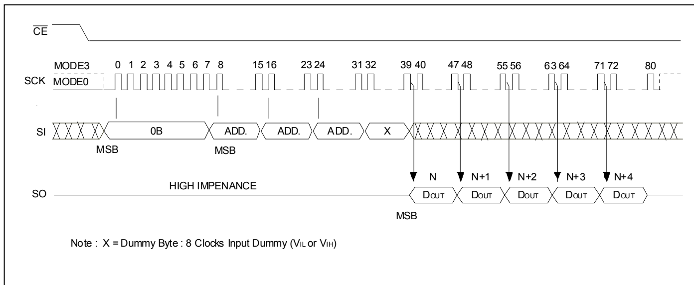
Figure 3 : HIGH-SPEED-READ SEQUENCE
