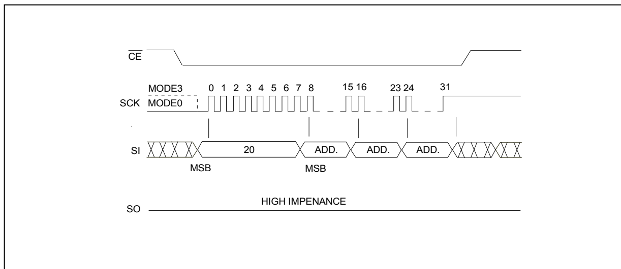
FIGURE 10 : SECTOR-ERASE SEQUENCE
