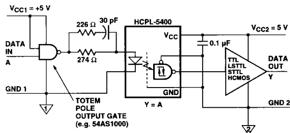
Figure 13. Recommended HCPL-5400 Interface Circuit.
