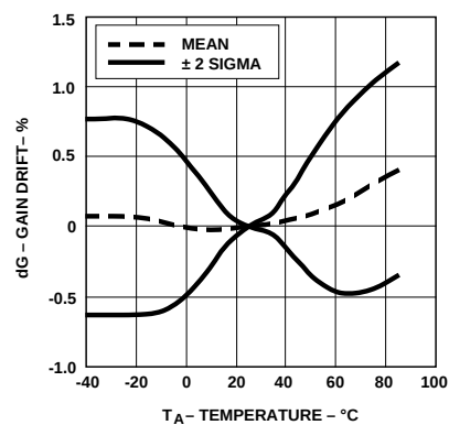
Figure 6. Gain Drift vs. Temperature.
