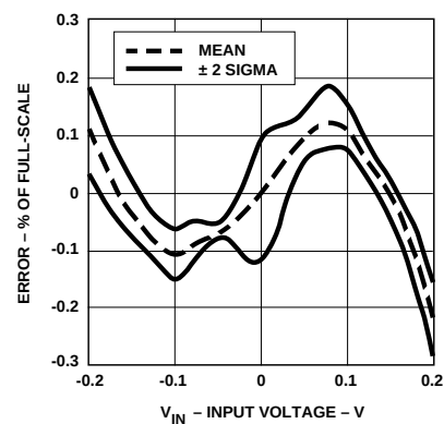
Figure 9. 200 mV Nonlinearity Error Plot.
