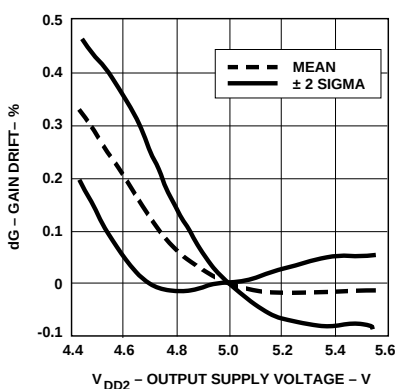
Figure 8. Gain Drift vs. V_{DD2} ( V_{DD1} = 5 V).
