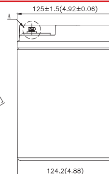
A Detail Drawing
