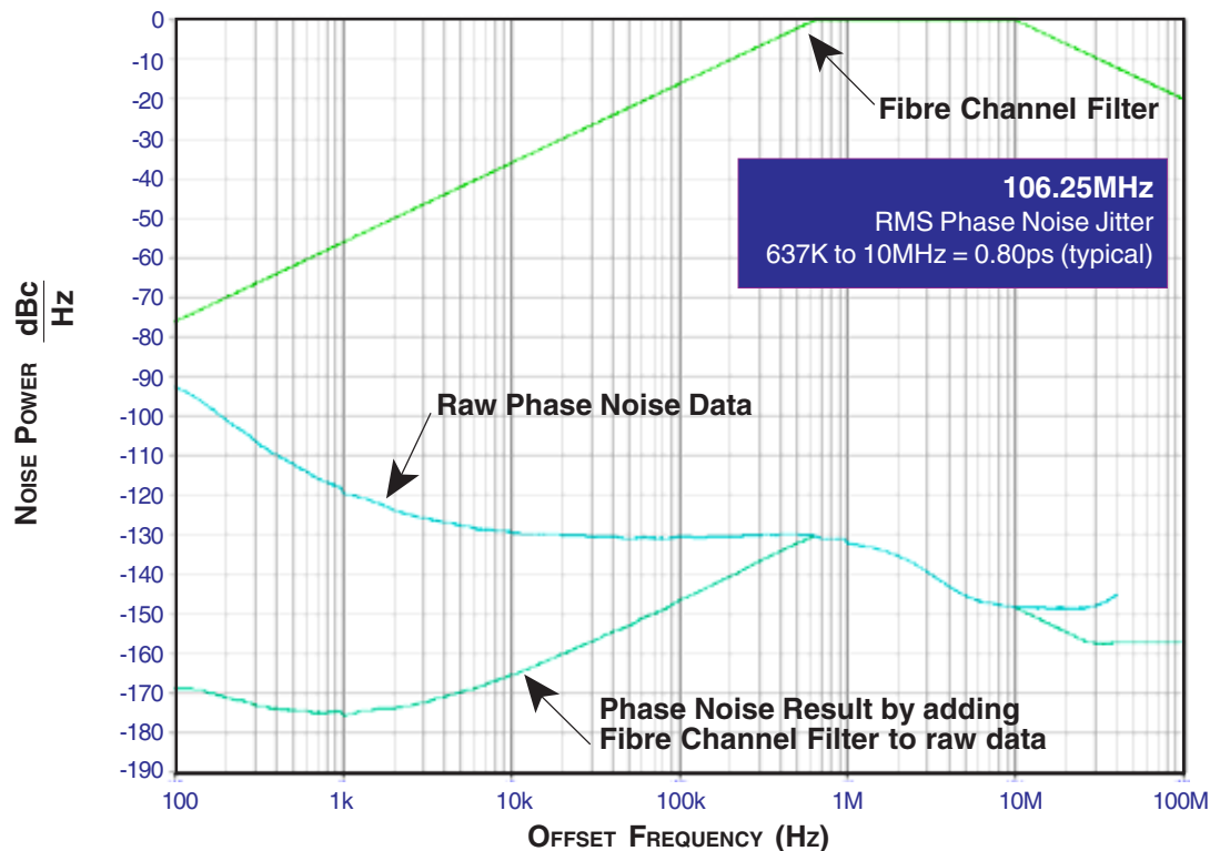
TYPICAL PHASE NOISE AT 106.25MHz
