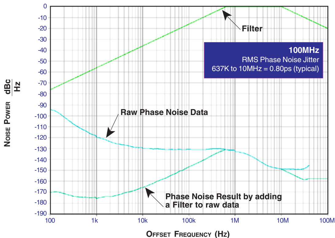
TYPICAL PHASE NOISE AT 100MHz
