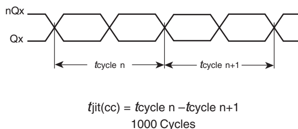
CYCLE-TO-CYCLE JITTER
